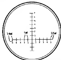
Figure 4-23. M19 binocular reticle.
